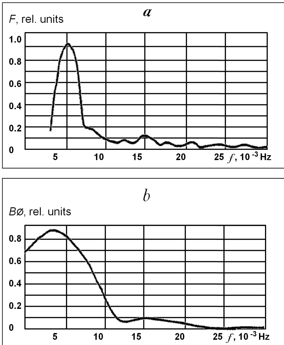
Figure 5. Frequency Spectra of the H-component of the Geomagnetic Disturbance During the Substorm on July 15, 2000 (a) and a Calculated Spectrum of the Signal from an Explosion at an Altitude of 300 km (K-3) (b). 2
